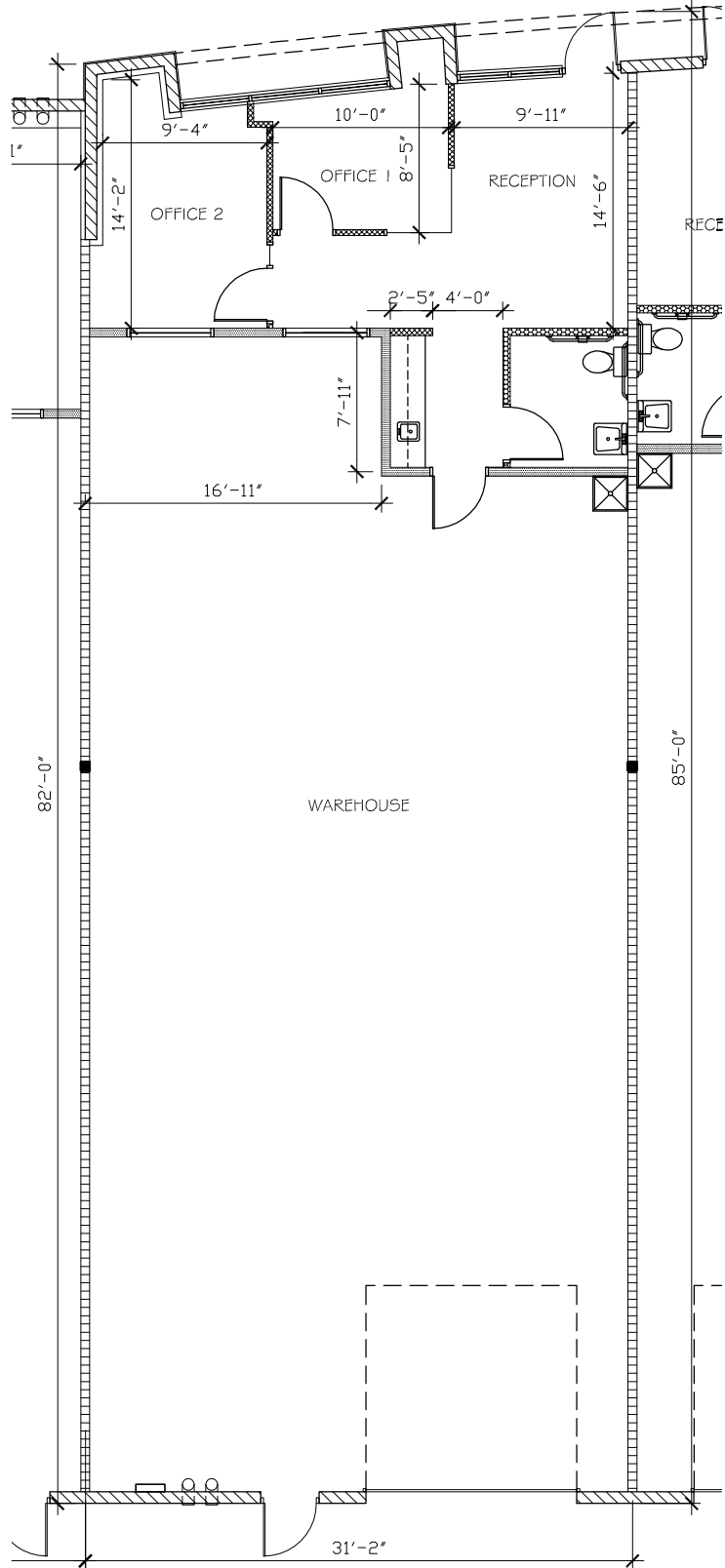
Bldg 'E' Suite 108 GROSS = 2608 SF USABLE = 525 SF OFFICE / 1928 SF WRHS
