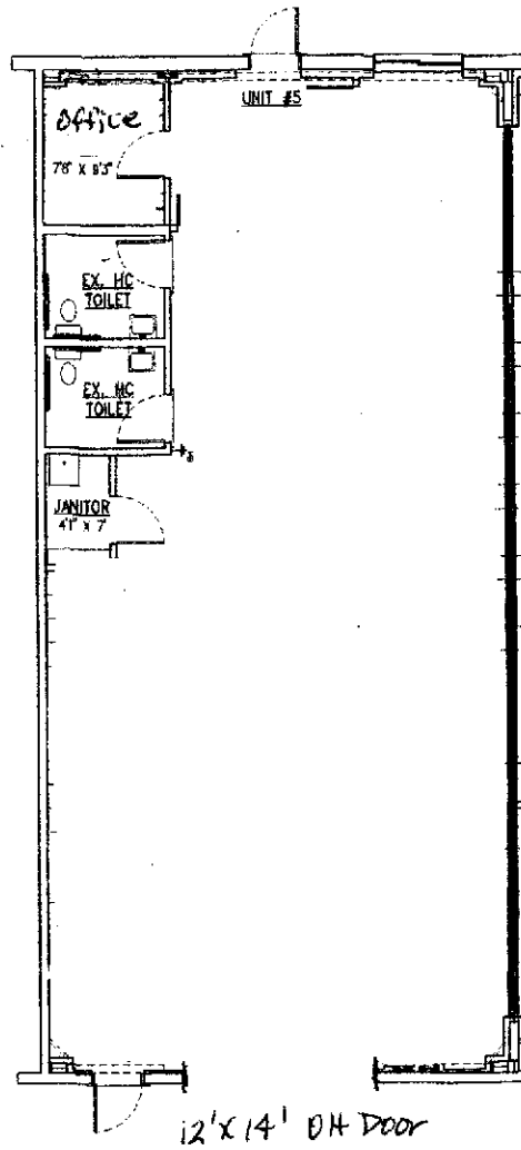
1 FIRST FLOOR PLAN - PROPOSED 1/4"=1'-0"
