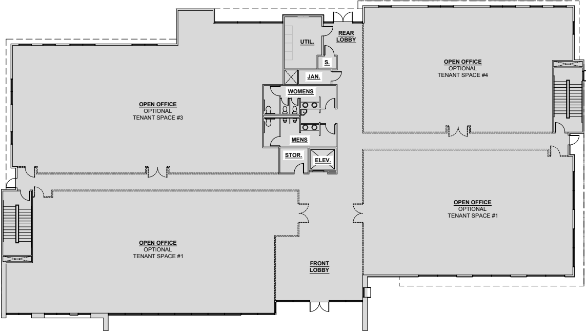
GROUND LEVEL FLOOR PLAN
