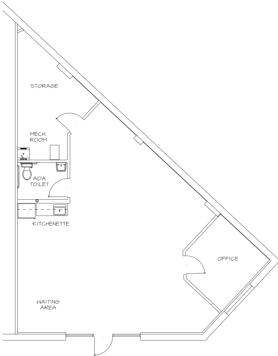
1 EXISTING FLOOR PLAN - 1,305 S.F. SCALE: 1/8" = 1'-0"
