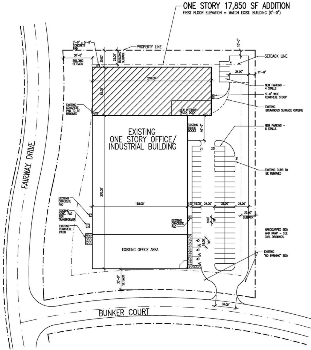
1 SITE PLAN A000 1" = 40' NORTH
