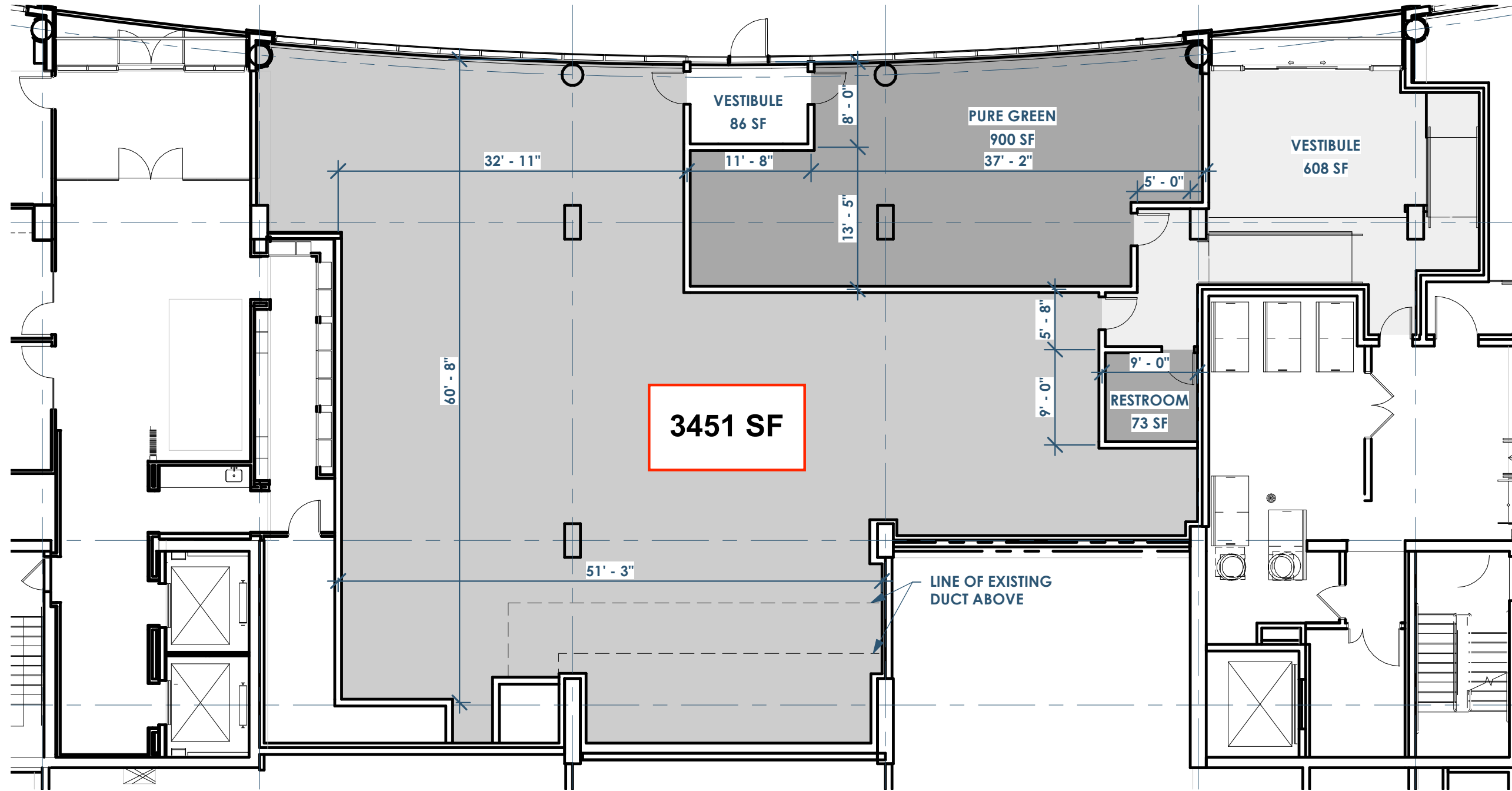
A1/O2 FLOOR PLAN - 1ST FLOOR - OPTION 2 3/32" = 1'-0"
