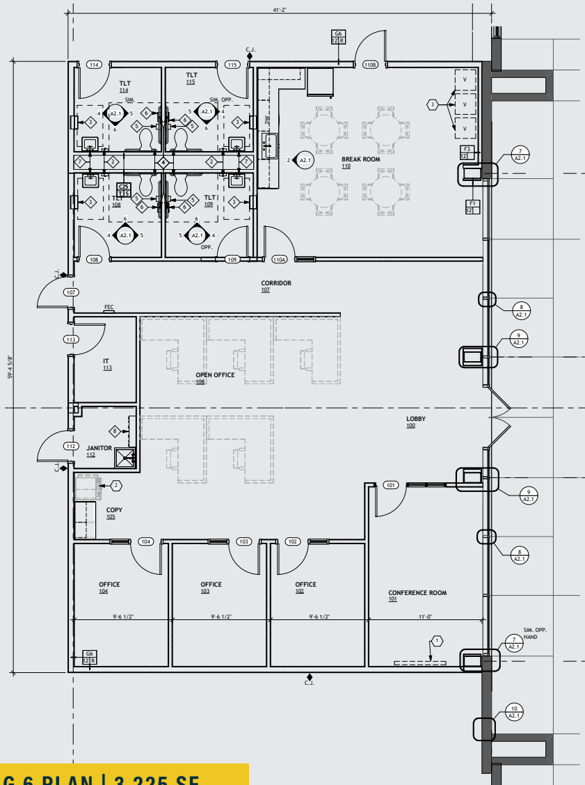
BUILDING 6 PLAN | 3,225 SF
