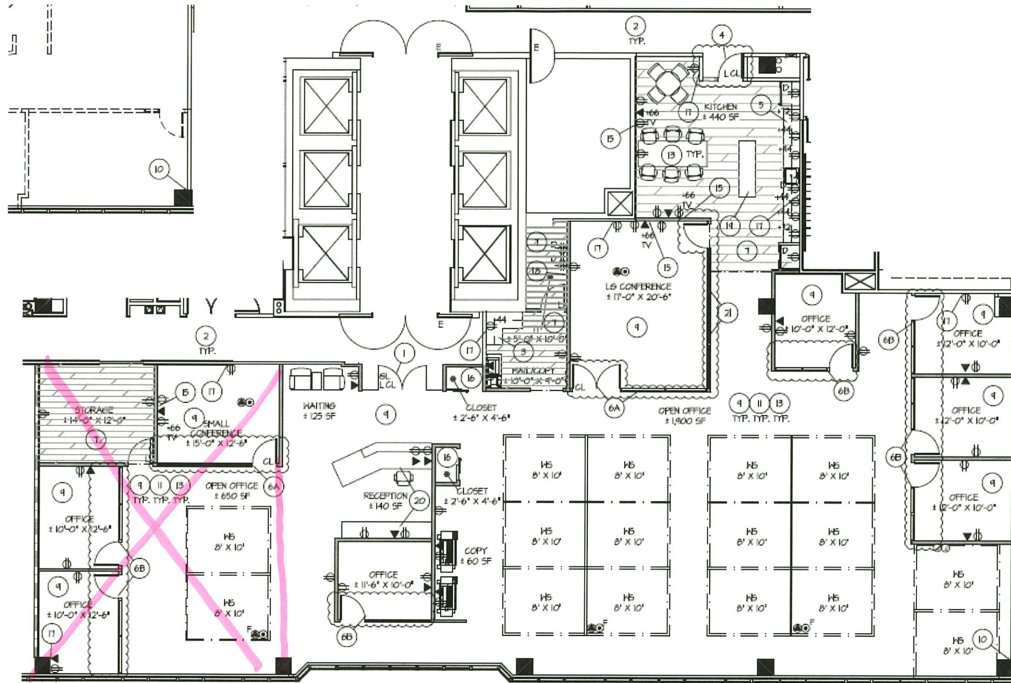
○ SUITE 750 - NEW FLOOR PLAN
