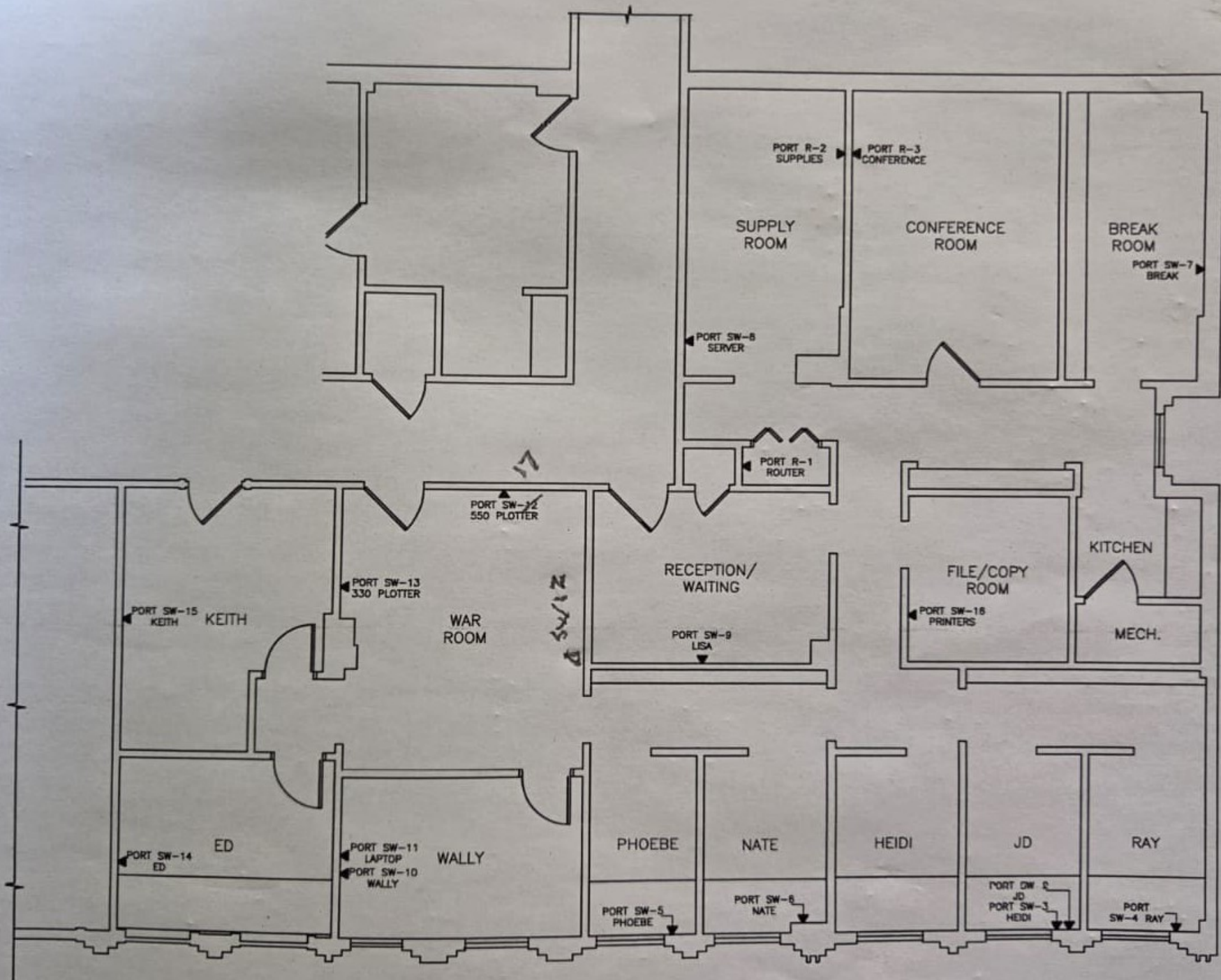
OFFICE NETWORK LAYOUT 1/8"=1'-0"
