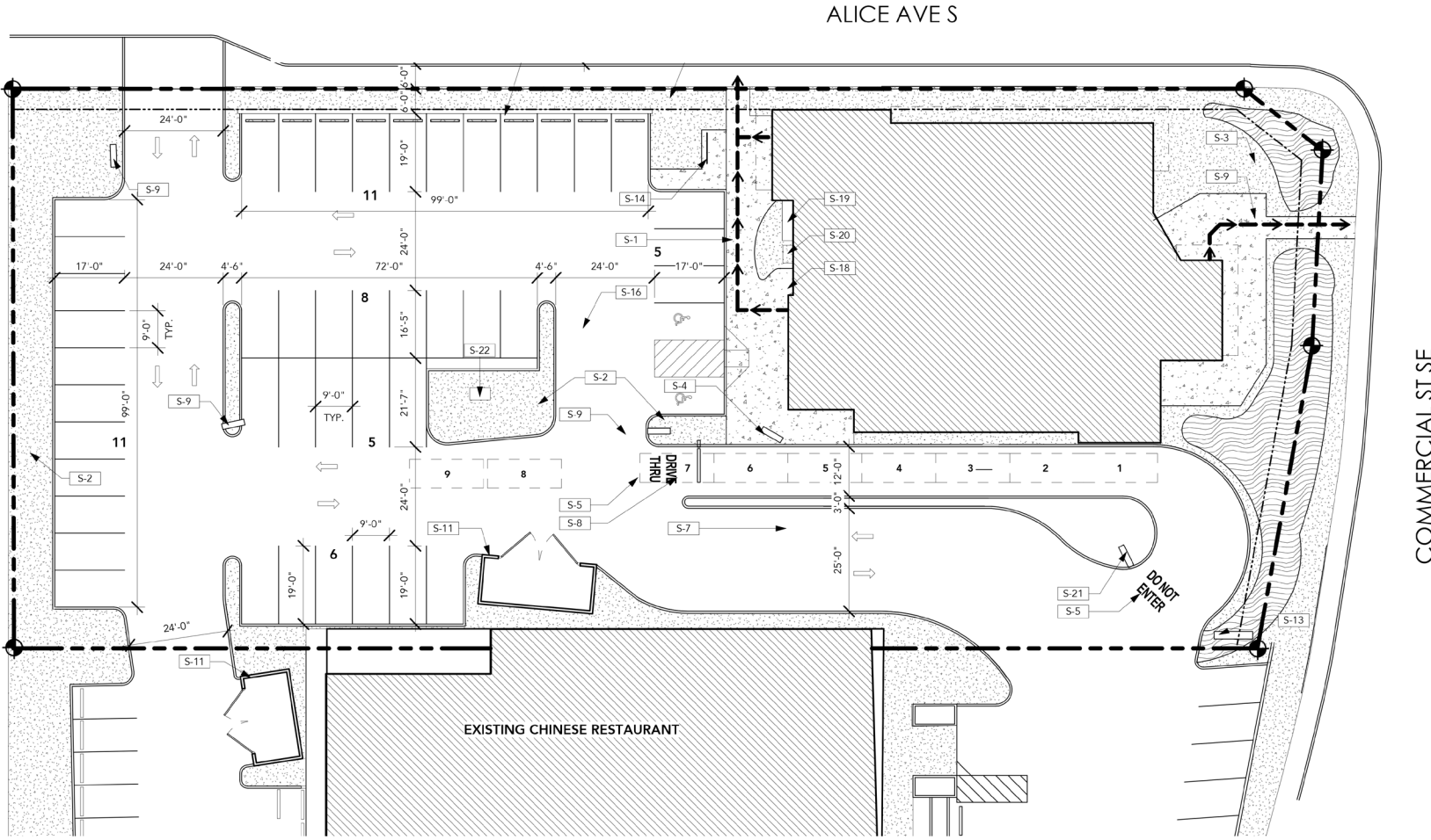
1 SITE PLAN 1" = 20'-0"
