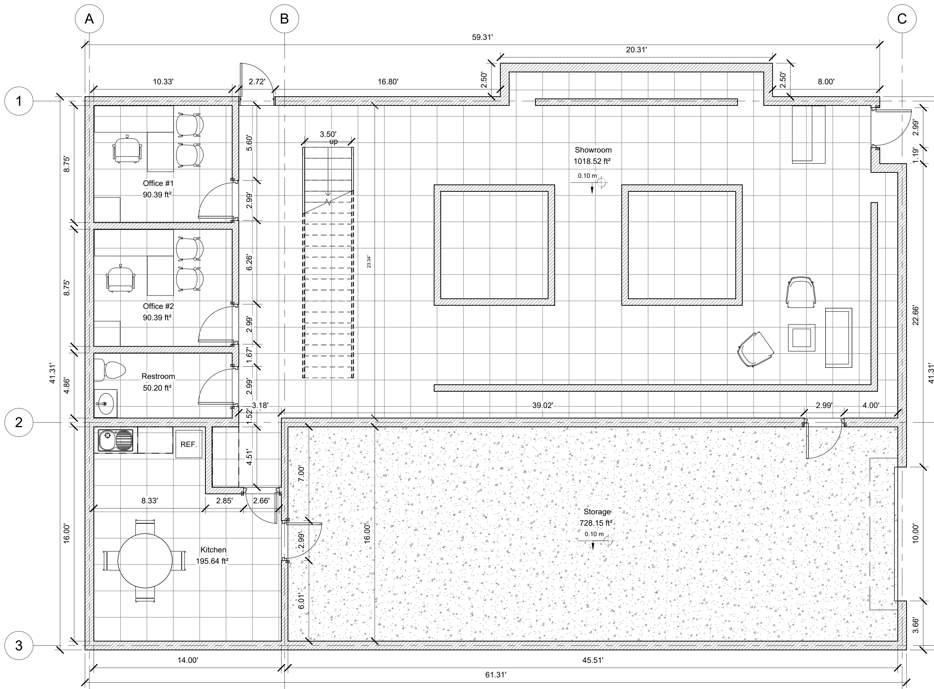
A1 1st Level Floor Plan 1 : 50
