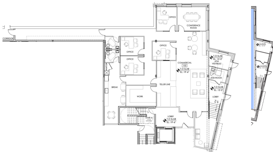
FIRST FLOOR CONCEPTUAL PLAN 1.0
