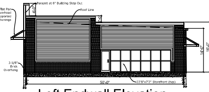
Left Endwall Elevation
