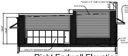
Right Endwall Elevation
