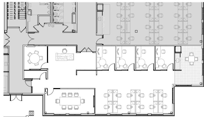
ENLARGED PLAN. SCALE: 3/32" = 1'-0"
