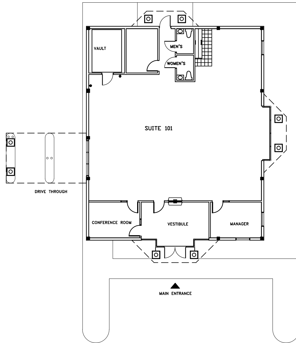
1 FIRST FLOOR PLAN ( AREA=3036 SQ.FT.) SCALE_1"=16'-0"
