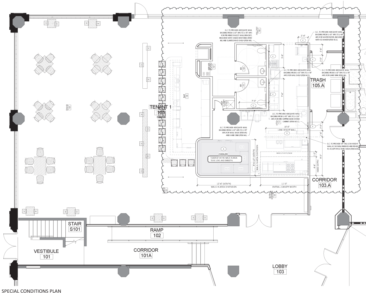
SPECIAL CONDITIONS PLAN SCALE: 1/8" = 1'-0"
