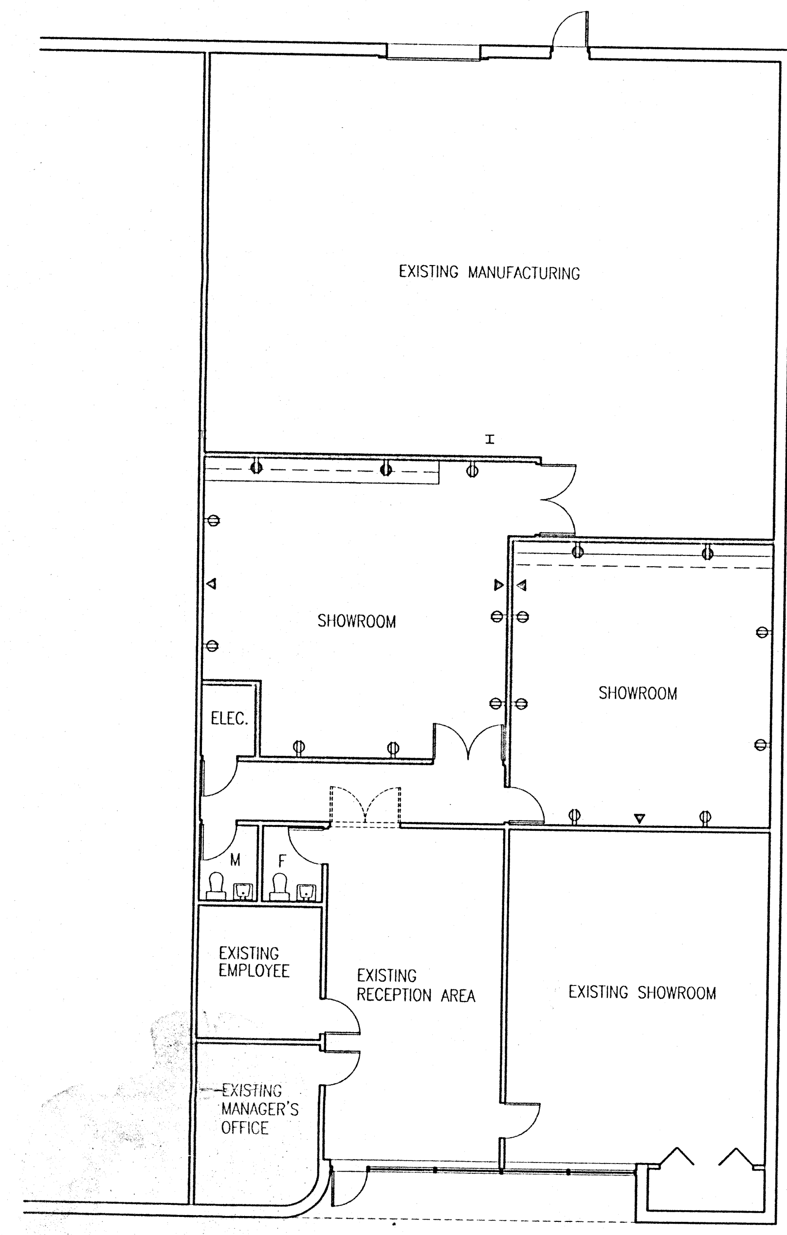
POWER WIRING PLAN SCALE 1/8" = 1'-0"
