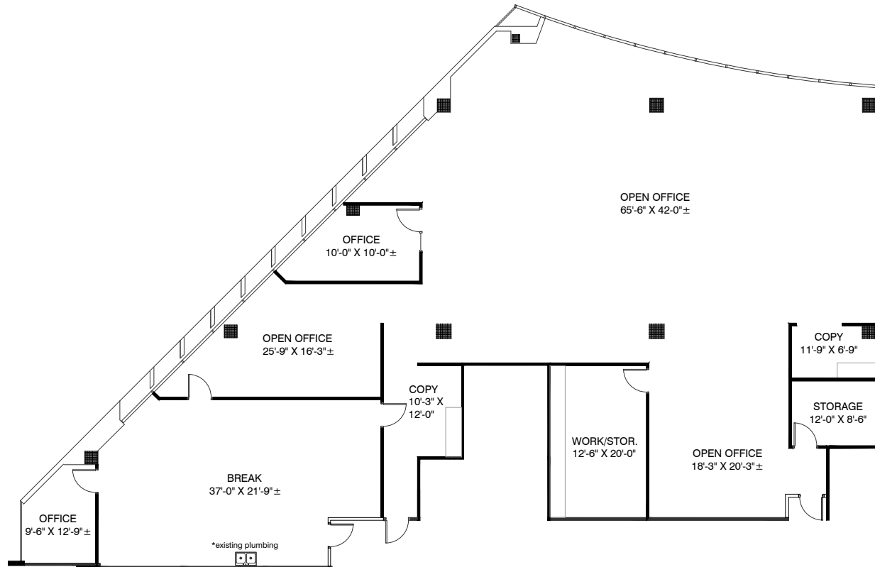
KEYPLAN - 7TH FLOOR
