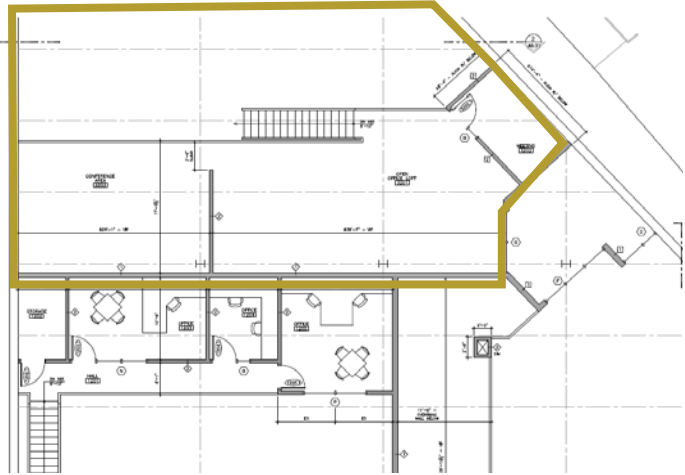
LOFT FLOOR
