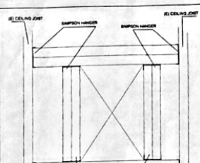
TYPICAL OPENING DETAIL N.T.S.
