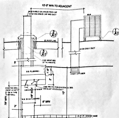
KITCHEN SECTION SCALE: 1/4" = 1'-0"
