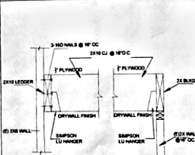
TYPICAL OPENING DETAIL N.T.S.
