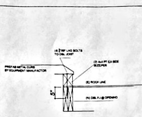
EXHAUST BLOWER BASE NTS
