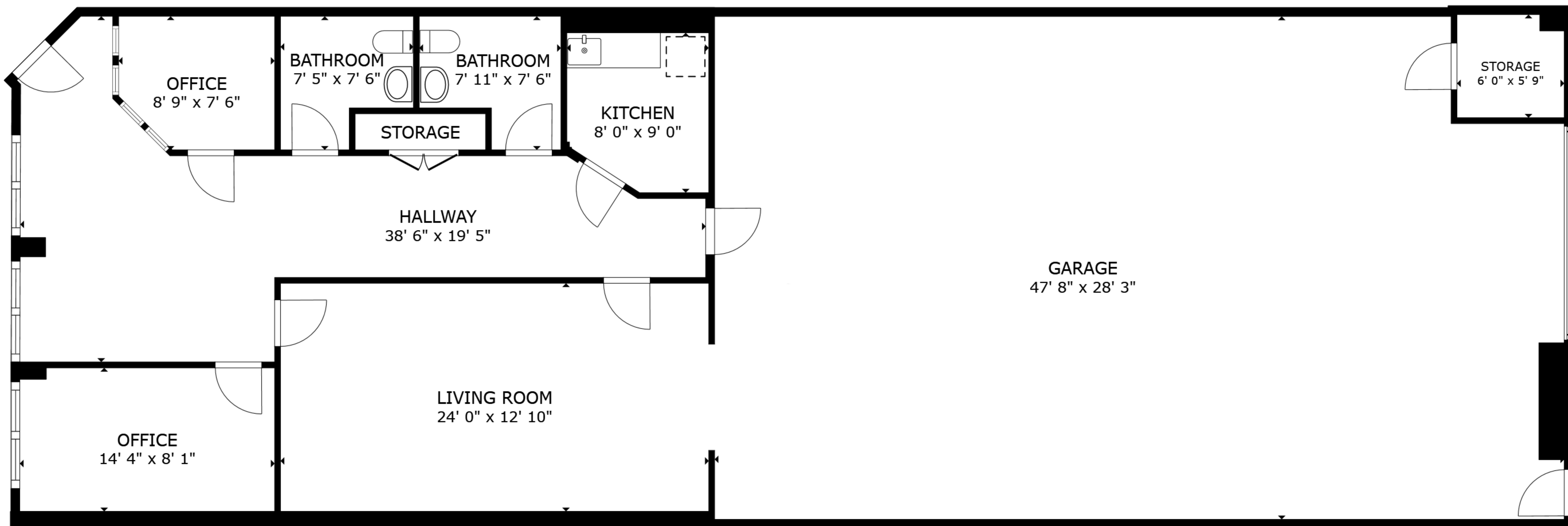
FLOOR PLAN
