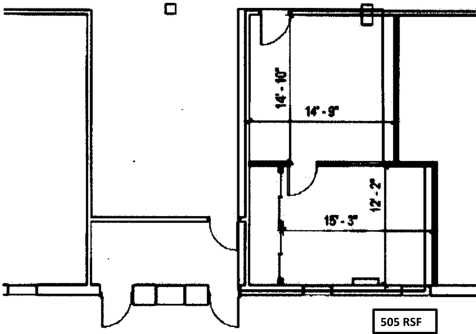
First Floor Plan- Suite #112
