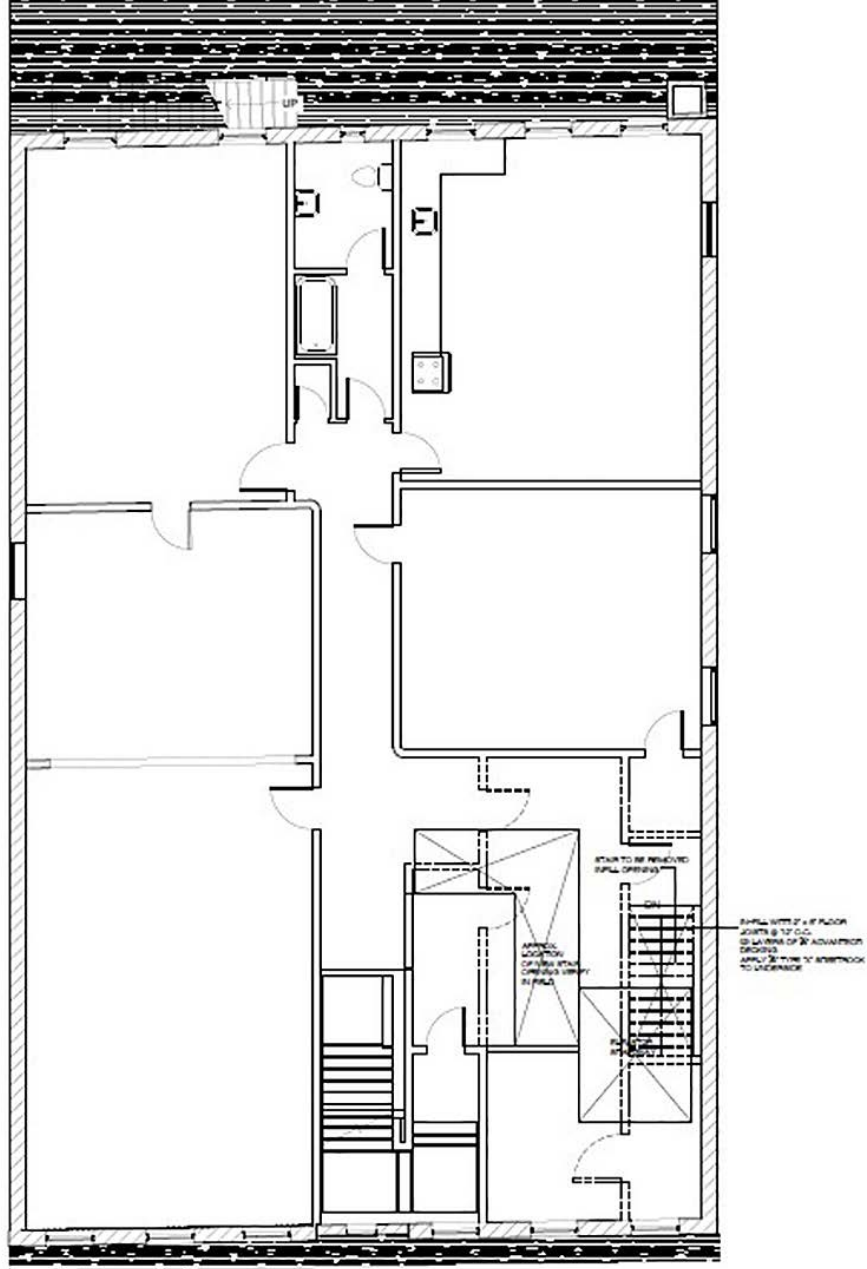
SECOND FLOOR PLAN - EXISTING
