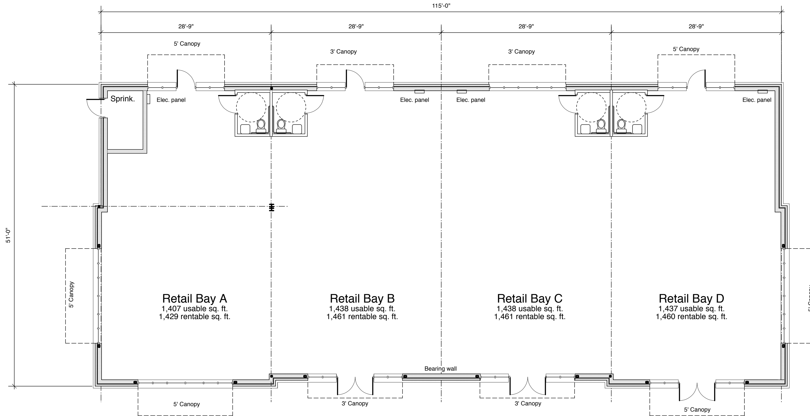
Floor Plan
