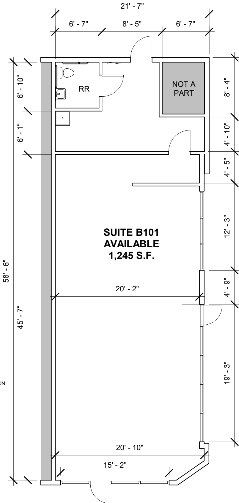
1 DIMENSION PLAN B101 1/8" = 1'-0"
