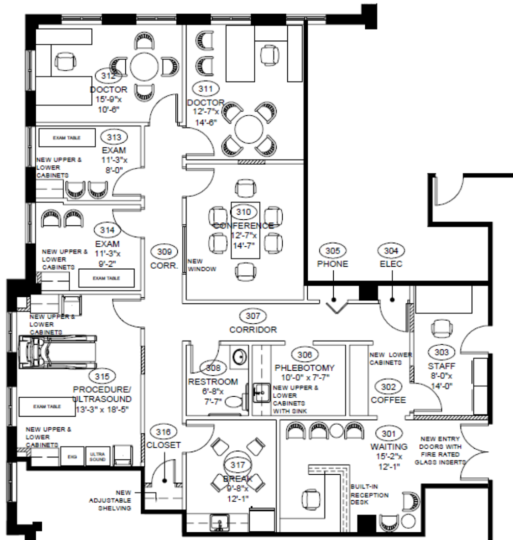
KEY PLAN
