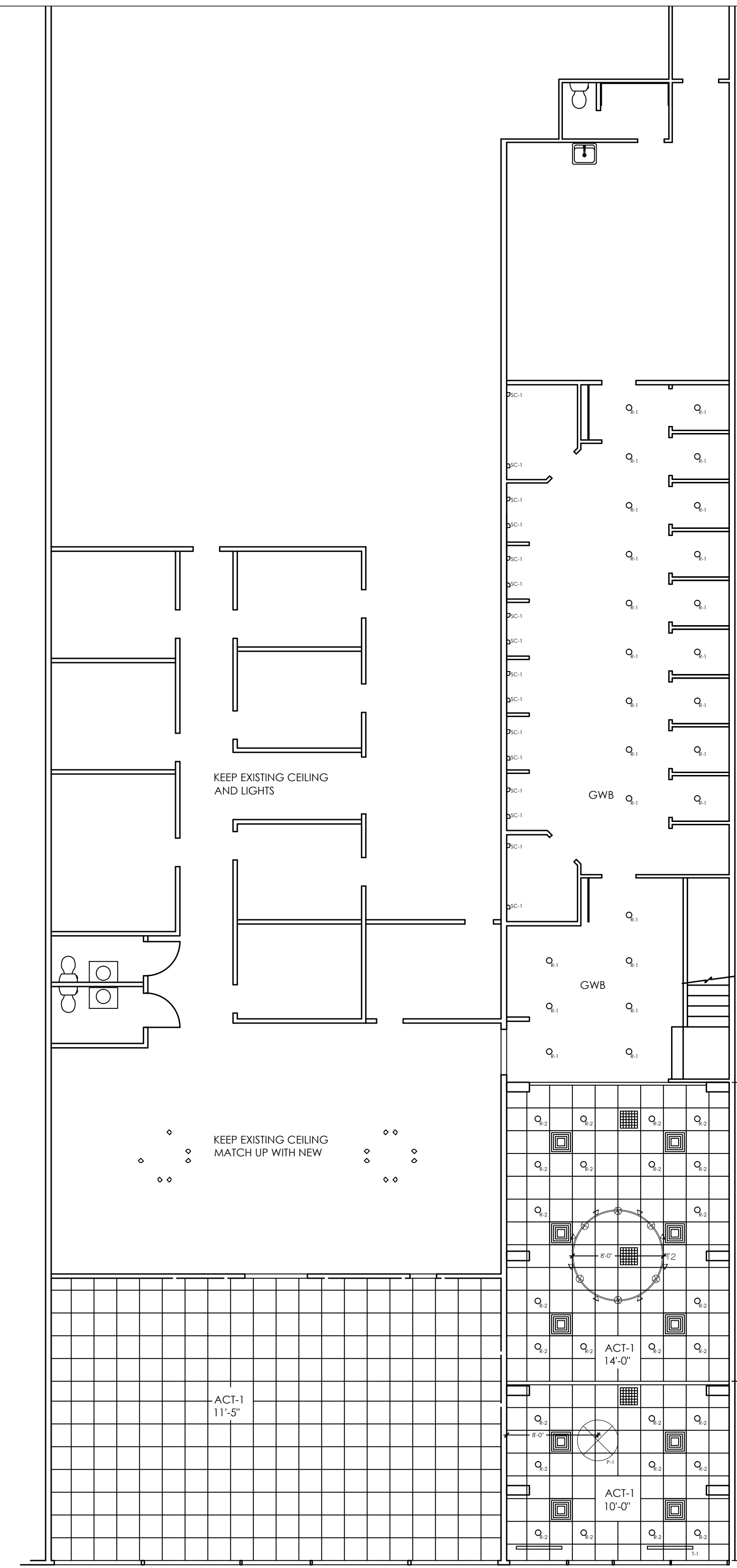
CEILING & LIGHTING PLAN
