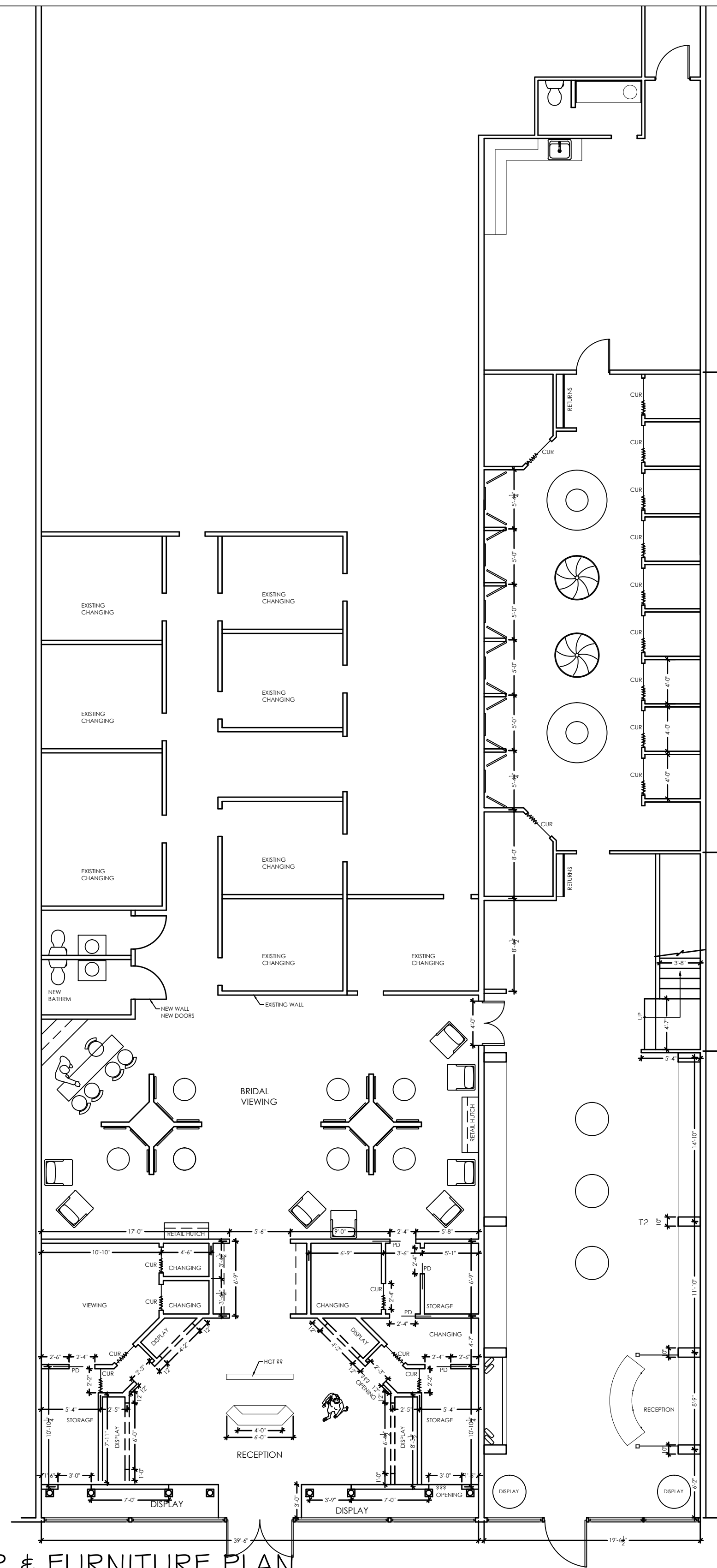
FLOOR & FURNITURE PLAN
