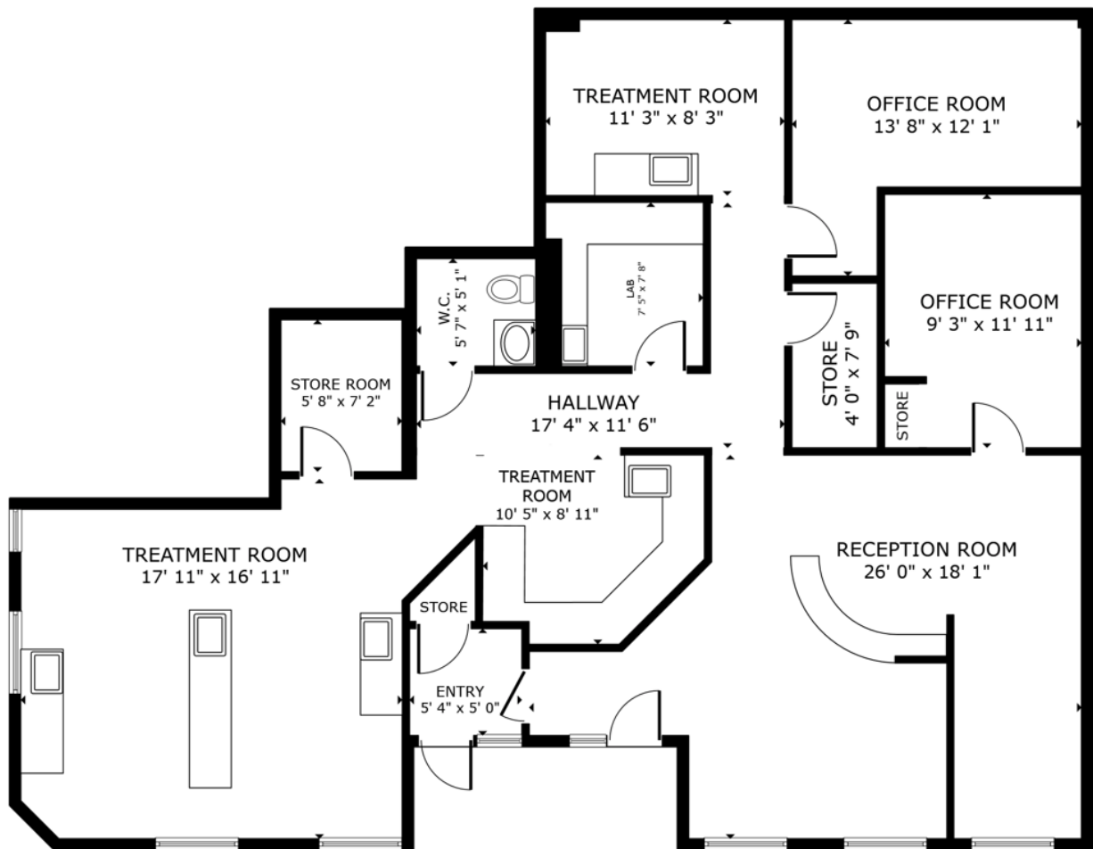
FLOOR PLAN
