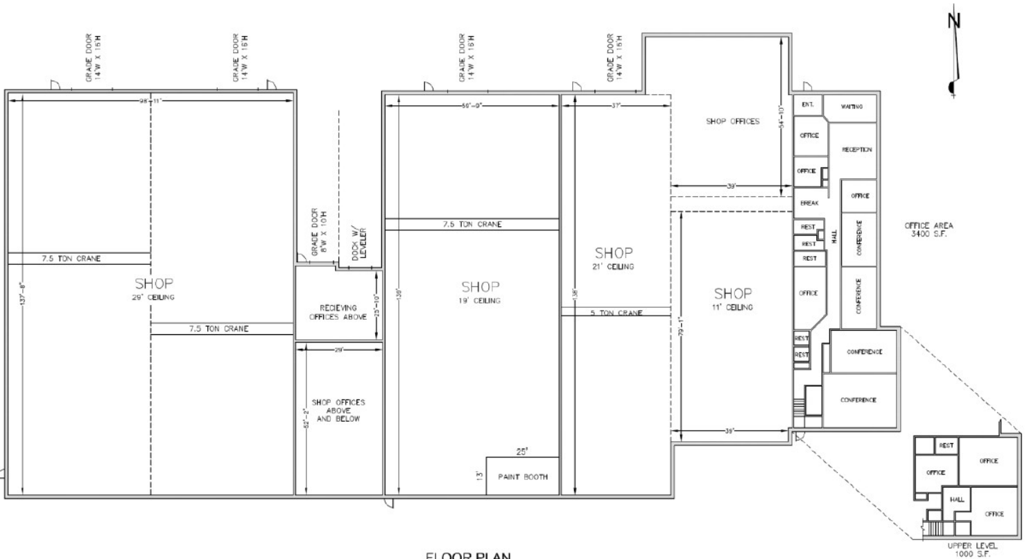
FLOOR PLAN 6202 S. STATE ROAD GROSS AREA 40,000 S.F.
