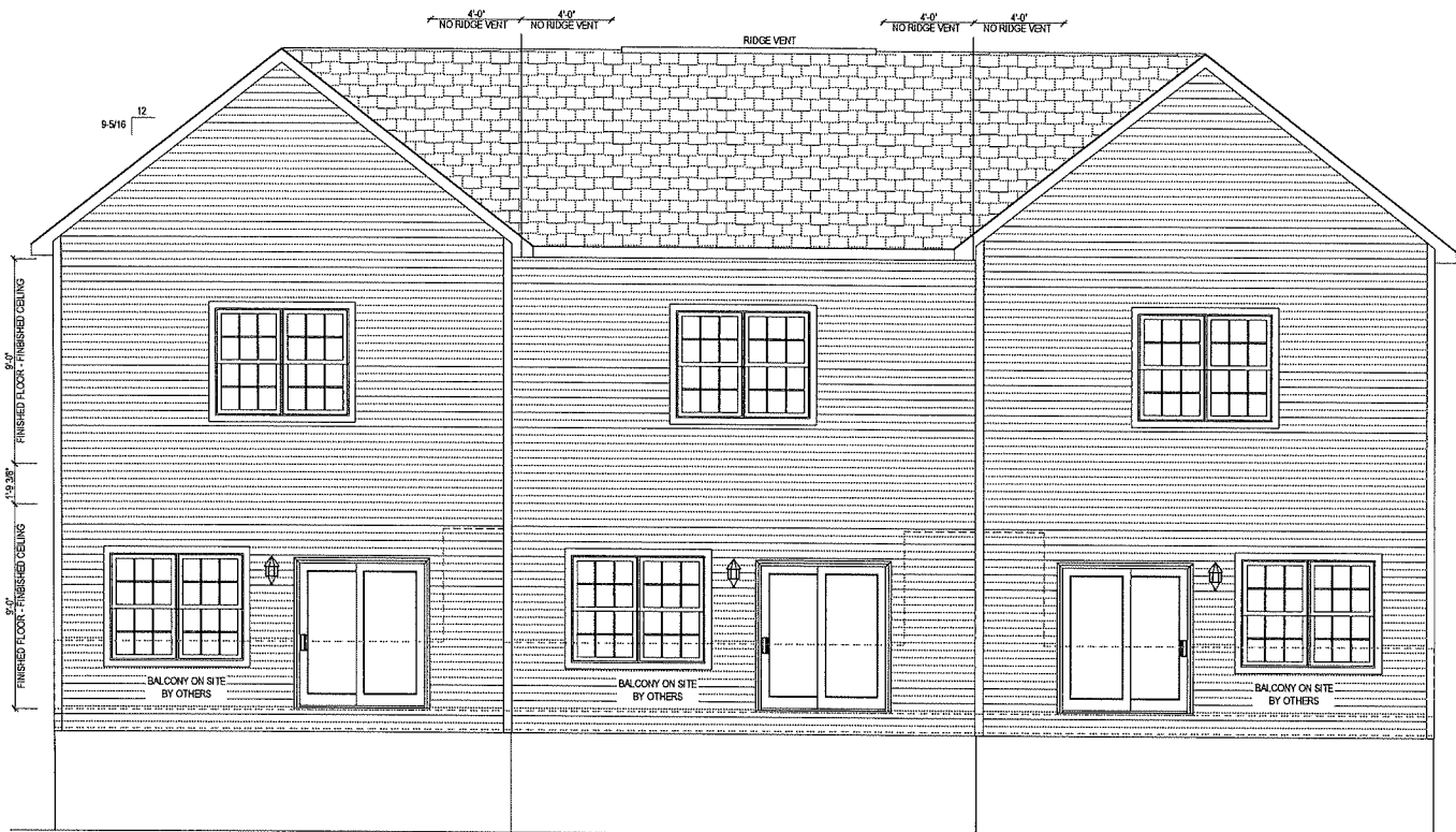
REAR ELEVATION
