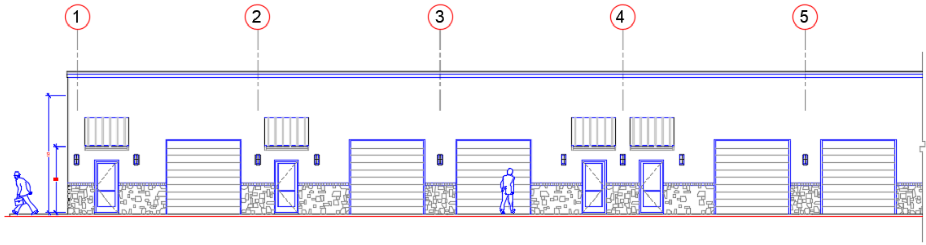
SOUTH ELEVATION
