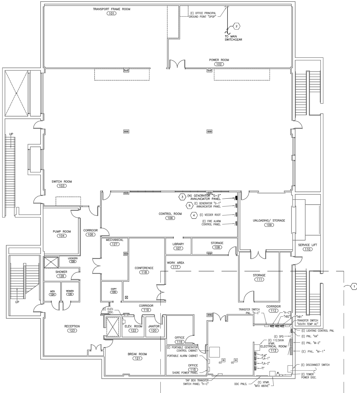
1 BASEMENT PLAN - NEW WORK 1/8" = 1'-0"
