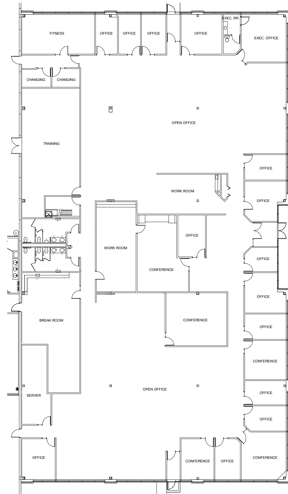
1 EAST OFFICE || 17,692 SF 3/64" = 1'-0"
