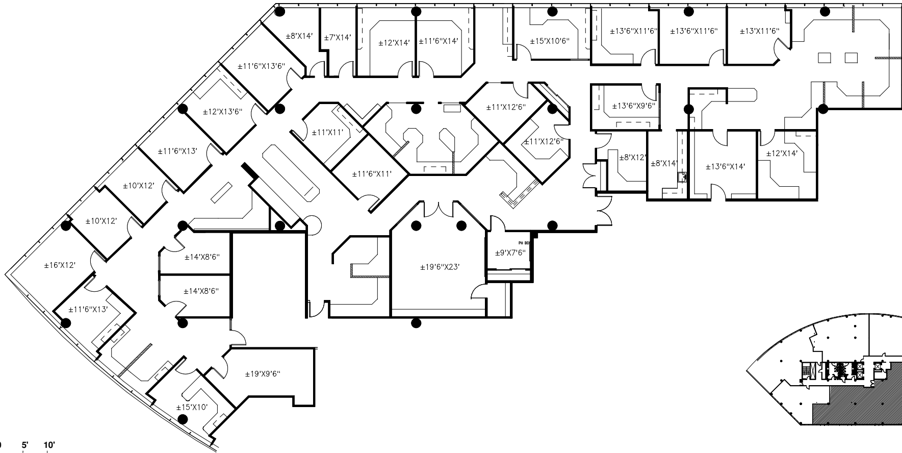
KEY PLAN
