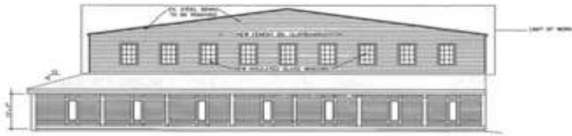
WEST ELEVATION ② 1/8"=1'-0"
