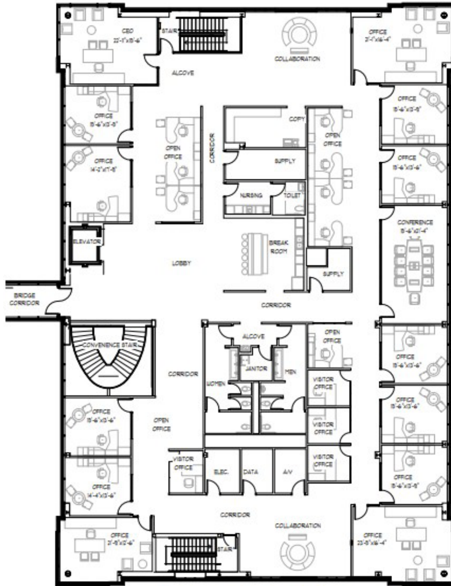
1 THIRD FLOOR EXISTING PLAN A-4 SCALE: 1/16" = 1'-0"
