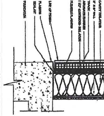
EIFS WALL SECTION SCALED
