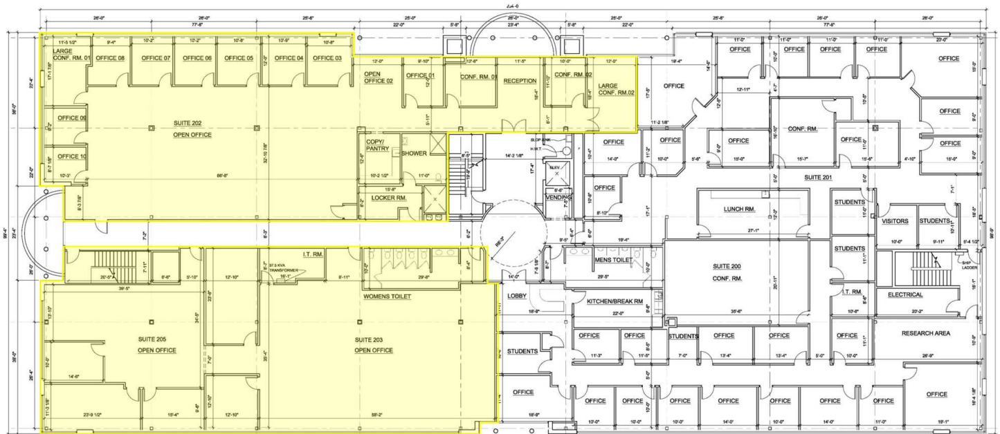
1 1.2 EXISTING SECOND FLOOR PLAN 1/8" = 1'-0"
