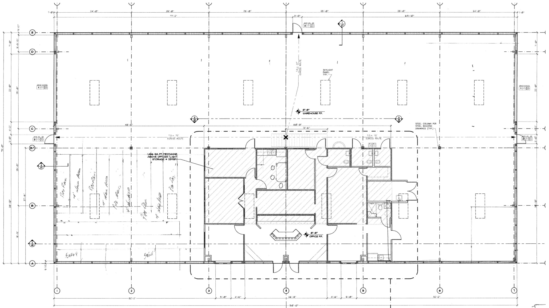
FLOOR PLAN 3/16"=1'-0"
