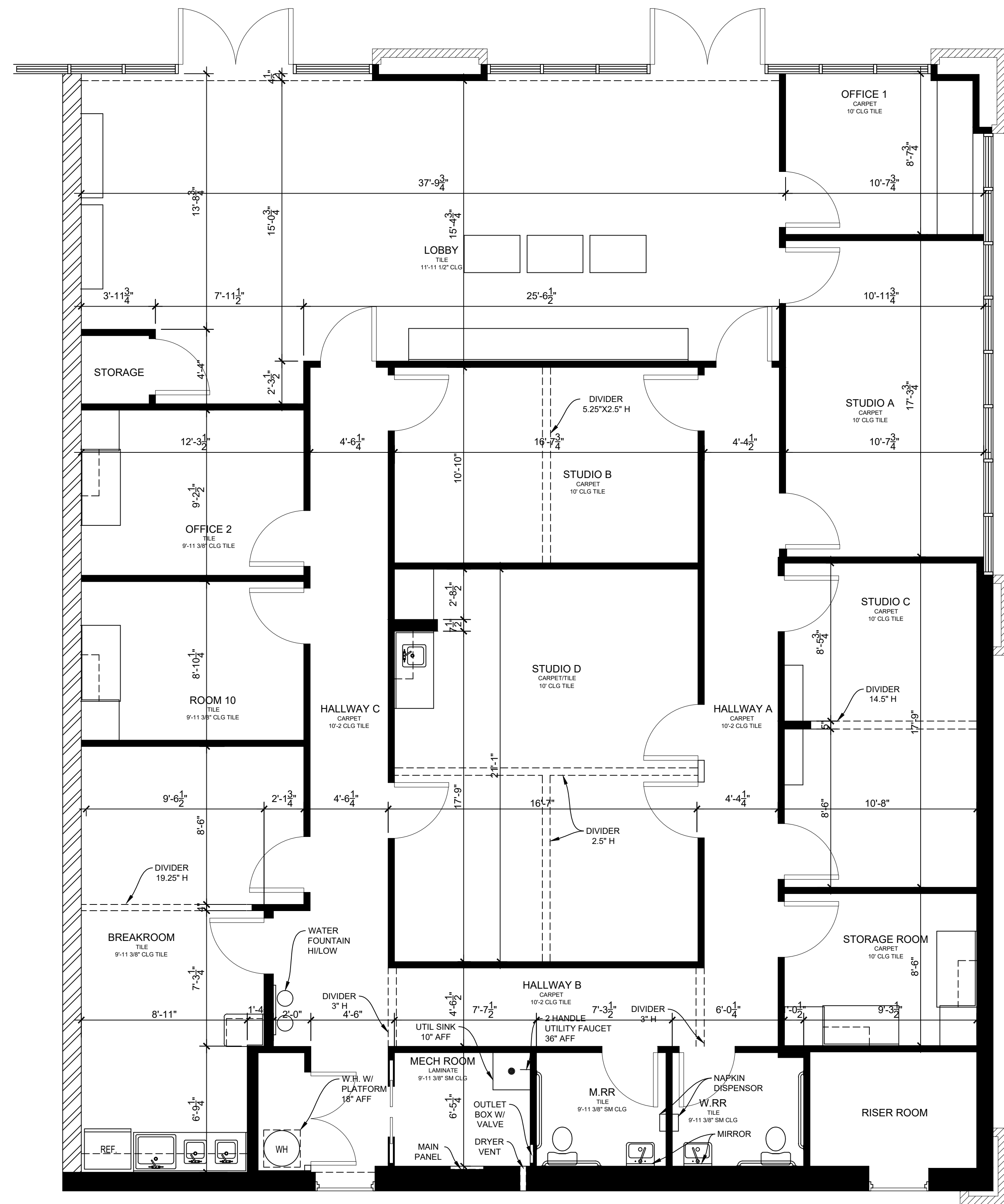
EXISTING FLOOR PLAN / SCALE: 1/4"=1'-0"
