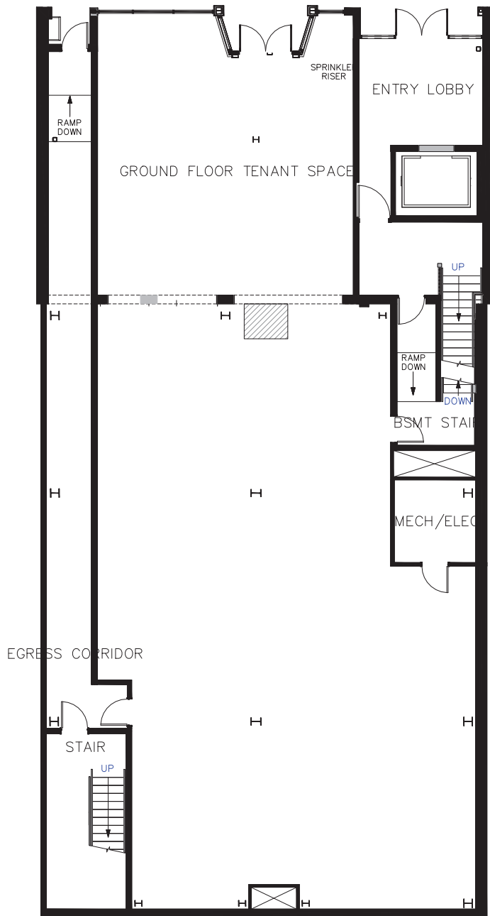
1ST FLOOR PLAN 3,780 SF
