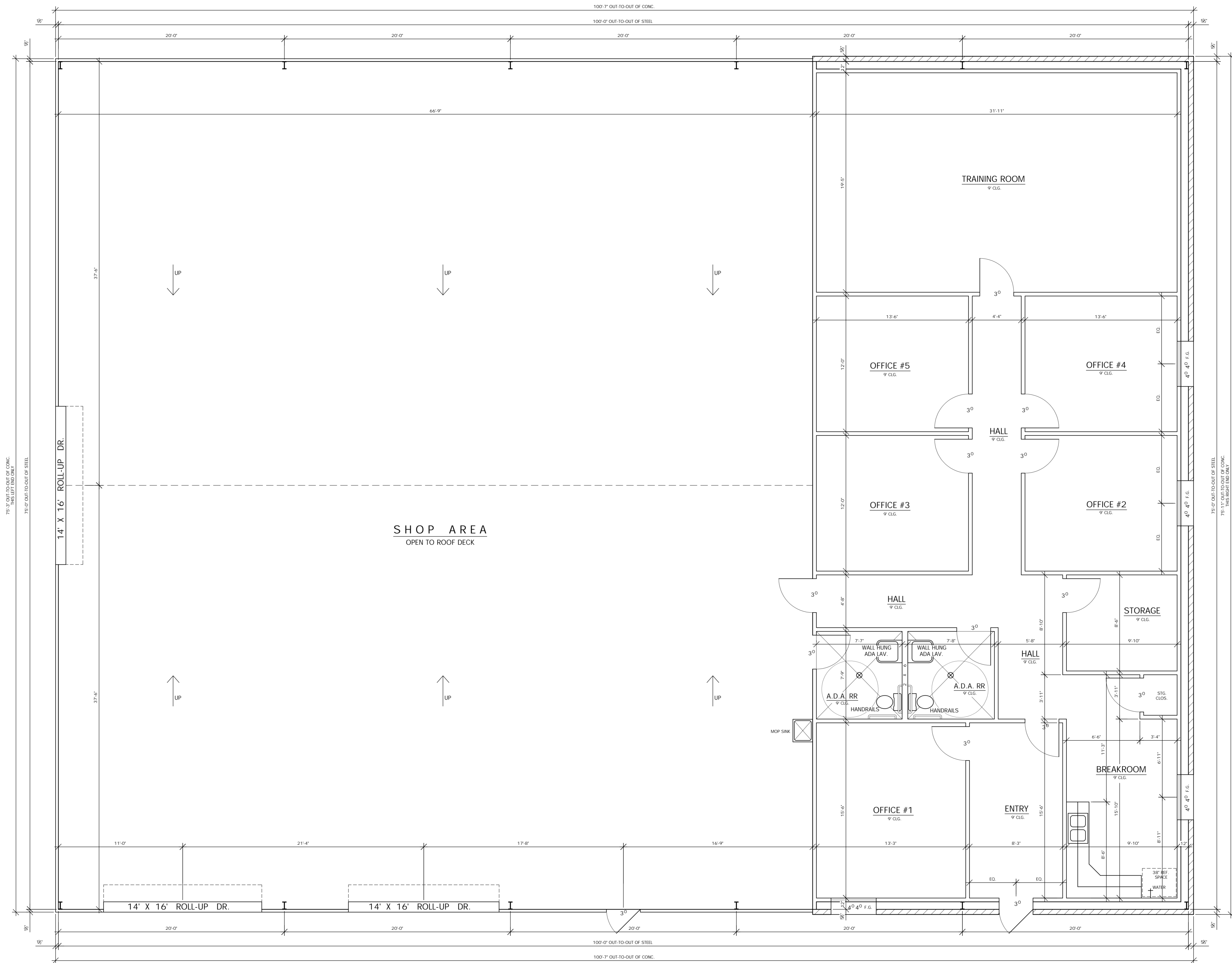
FLOOR PLAN SC: 1/4" = 1'-0" APPROX. 7500 SQ.FT.
